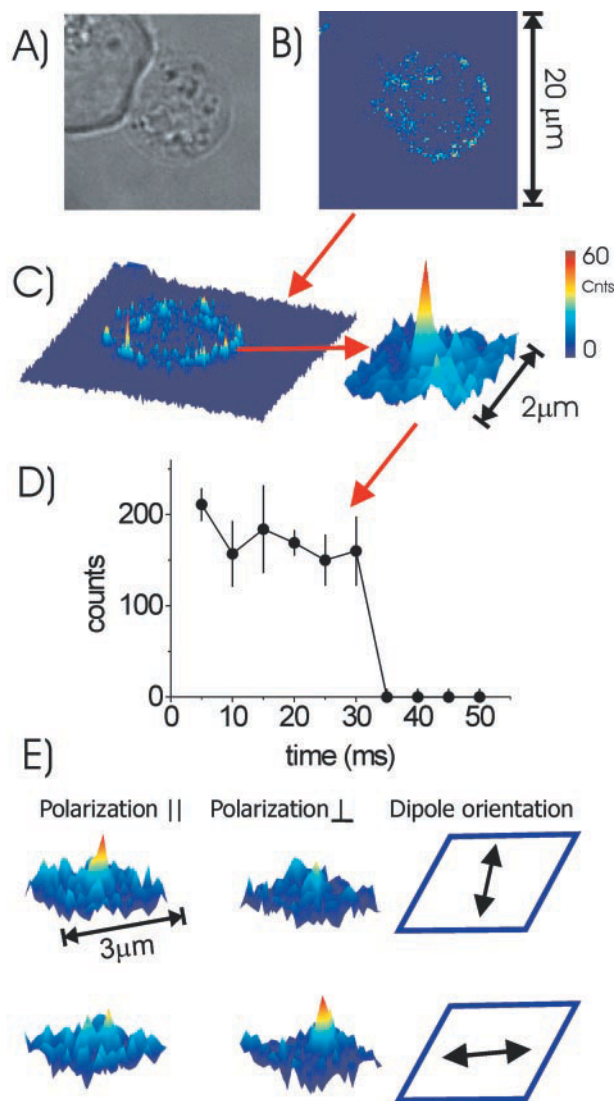
FIGURE 3 Single-molecule characterization. (A) White light and (B) fluorescence image of an HEK293 cell transfected with eYFP- \alpha_{1C,77} subunits of a \text{Ca}^{2+} channel. (C) Enlarged fluorescence image. (D) The mean detected fluorescence attributable to an individual eYFP- \alpha_{1C,77} is 34 cnts/ms. After 6 observations, a single-step photobleaching event occurred. (E) Polarization images taken at an interval of 110 ms showing a slow rotation of an individual eYFP- \alpha_{1C,77} (the excitation light was circularly polarized). Only two images of a series are shown. It should be noted that such slow rotation was found for only 10% of all signals observed. The angles of the transition-dipole moment (boxed arrows) with respect to the laboratory coordinates were determined from the intensity ratio in the parallel ( \parallel ) and perpendicular ( \perp ) directions. All fluorescence images are scaled between 0 (blue) and 60 cnts/pxl (red).
