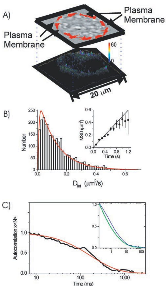
FIGURE 5 \text{Ca}^{2+} channel mobility. (A) Ensemble of single-molecule trajectories (red lines) overlaid by a white-light image of an HEK293 cell. All trajectories are confined to the cell's perimeter. The fluorescence images are scaled between 0 (blue) and 60 cts/pxl (red). (B) Distribution of lateral diffusion constants, D_{\text{lat}} , of 2492 individual eYFP- \alpha_{1C,77} on the cell surface. The distribution has a mean of D_{\text{lat}} = 0.15 \mu\text{m}^2/\text{s} . For a linear analysis, a deviation from normal diffusion behavior does not occur up to a length scale of 0.7 \mu\text{m} (inset). (C) Signal obtained by fluorescence correlation spectroscopy of eYFP- \alpha_{1C,77} \text{Ca}^{2+} channel subunits in HEK293 cells. Only correlation events longer than 50 ms were analyzed (see Methods). Fitting of the data to a 2-D diffusion model (red curve) yielded a diffusion time of 200 ms, which corresponds to a diffusion constant of 0.11 \mu\text{m}^2/\text{s} . Photobleaching events of a fraction of molecules between 50 and 600 ms likely account for the jaggedness of the correlation curve. Inset: Comparison with fluorescence correlation curves of nonfused eYFP in the cytosol of HEK293 cells (blue) and purified eYFP in phosphate-buffered saline (green).
