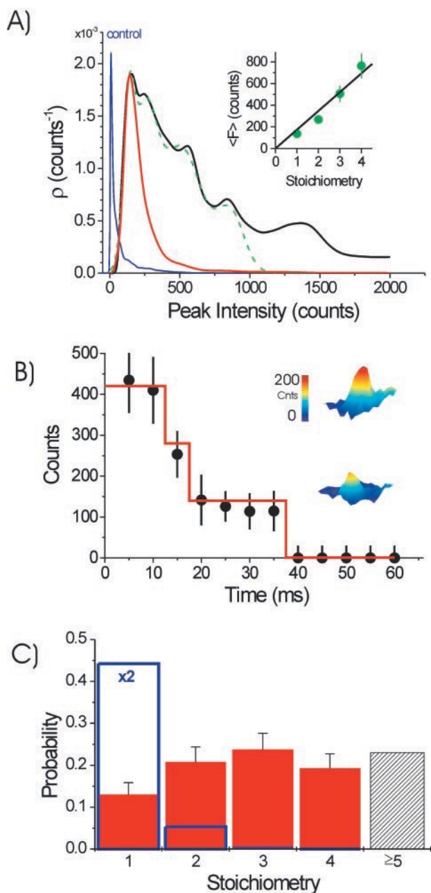
FIGURE 4 \text{Ca}^{2+} channel clustering. (A) Probability density function, \rho , of the fluorescence signal constructed from 271 individual observations on the surface of an HEK293 cell. The distribution was fit for signal intensities <1000 cnts to 4 Gaussians (dotted green line). For comparison, the intensity distribution obtained from an untransfected cell ("control"), and the distribution from individual eYFP-his 6 :Ni 2+ -NTA chelated lipids in an artificial lipid membrane are shown (Harms et al., 2001) (red curve). The positions of the maxima in the distribution were equidistant with a slope of 168 cnts/5 ms (inset). (B) Intensity of individual signals as a function of time. For an eYFP- \alpha_{1C,77} cluster a multiple-step (three-step) photobleaching event was observed. The horizontal lines are taken from the fit in Fig. 4 A inset. All fluorescence images are scaled between 0 (blue) and 200 cnts/pxl (red). (C) Statistical analysis of the stoichiometry of all 3417 observed signals (solid column). Assuming an even distribution of eYFP- \alpha_{1C,77} with a density of 0.24 per resolution-limited area ( 0.08 \mu\text{m}^2 ), a Poisson distribution (open columns) is predicted.
